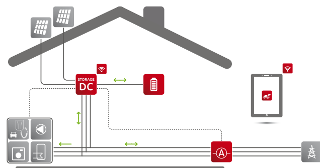
DC-SPEICHERSYSTEM RCT POWER STORAGE DC RCT POWER BATTERY RCT POWER SENSOR
