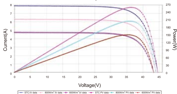
Module IV Graph 260W
