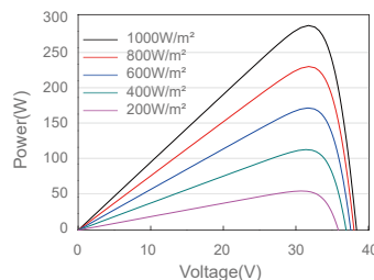
Power-Voltage Curve JAP6(K)-60-270/4BB
