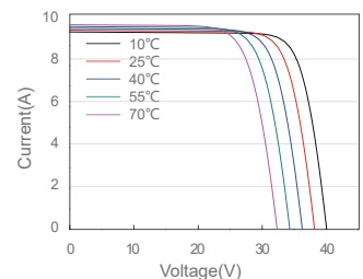
Current-Voltage Curve JAP6(K)-60-270/4BB
