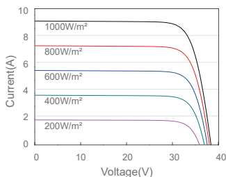
Current-Voltage Curve JAP6(K)-60-270/4BB
