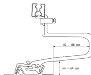
3D SL Alu XL
