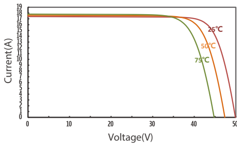
IV Curves of JT700SLk(B) at different Temp
