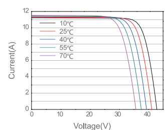
Current-Voltage Curve JAM60S21-365/MR
